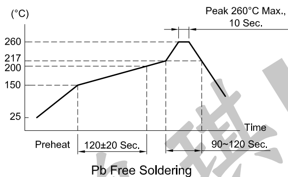
SOLDERING CONDITIONS
