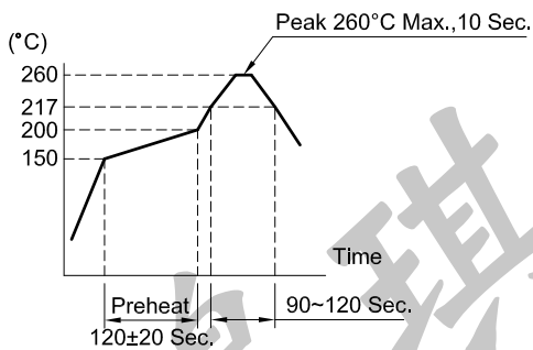
SOLDERING CONDITIONS
