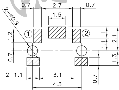
SOLDERING CONDITIONS
