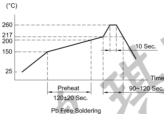
SOLDERING CONDITIONS
