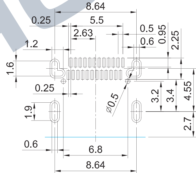
Pad Layout
