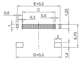
Pad Layout
