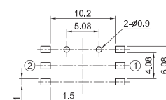
Pad Layout
