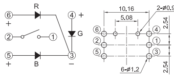
Circuit Mounting Hole Layout
