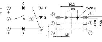
Circuit Pad Layout
