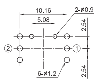
Mounting Hole Layout
