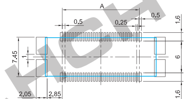
Pad Layout
