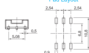
Pad Layout
