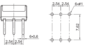
Mounting Hole Layout
