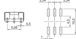
Pad Layout
