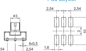
Pad Layout
